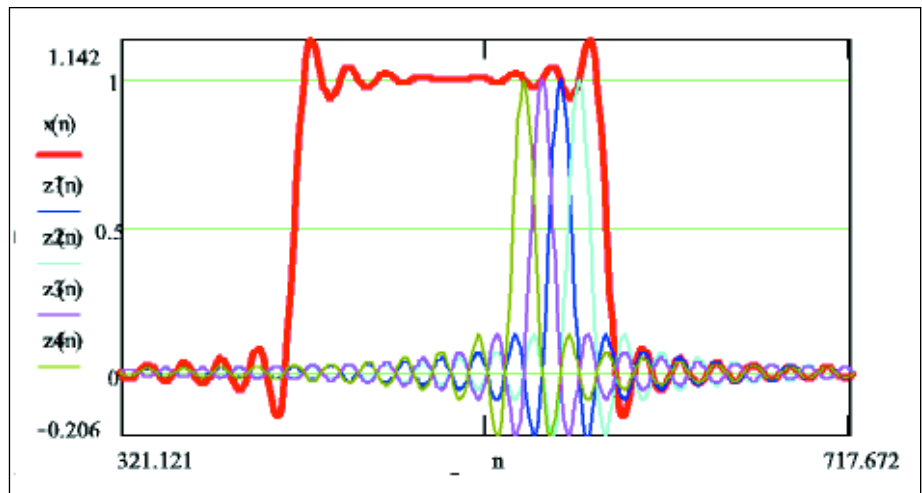
Figure 4. Overall spectrum of the simple OFDM signal shown with four subcarriers within. Note that the zero crossings all correspond to peaks of adjacent subcarriers.
