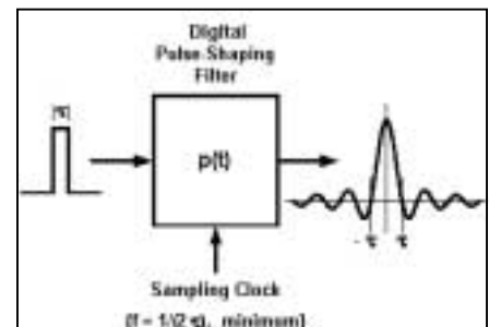
Figure 6. Converting an impulse to a raised cosine pulse by filtering.
