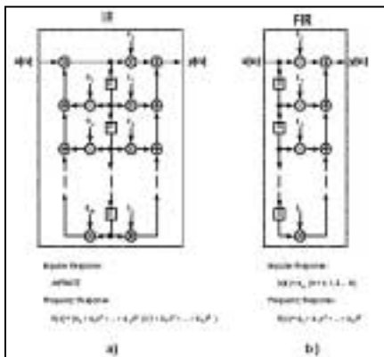
Figure 4. The functional form of FIR and IIR filters.
