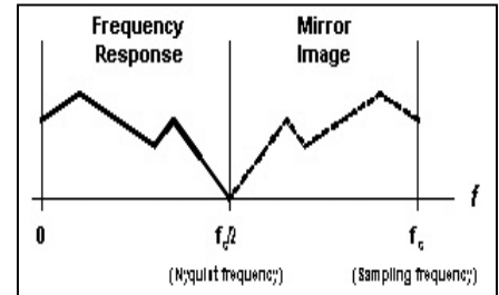
Figure 5. An arbitrary digital filter frequency response.
