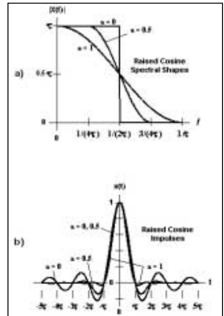
Figure 2. Spectral shape and inverse Fourier transform of the raised cosine pulse.
