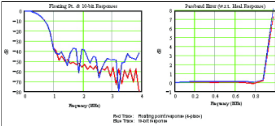
Figure 7. The frequency responses of two different versions of the raised cosine pulse-shaping filter.
