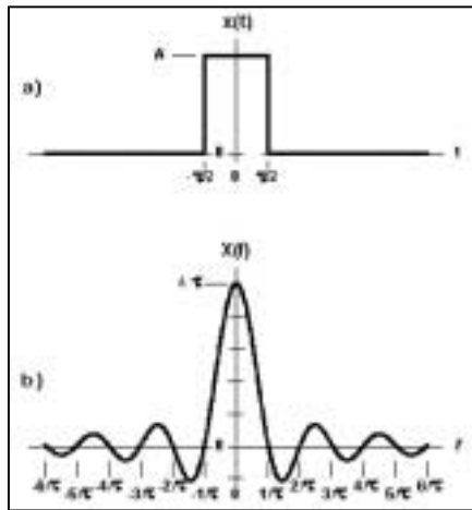
Figure 1. A single rectangular pulse and its Fourier transform.
