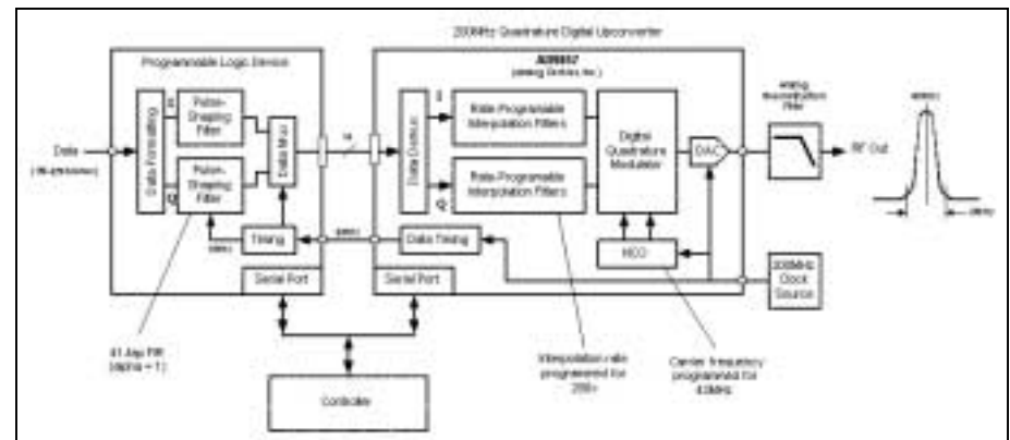
Figure 8. A block diagram of one potential RF data transmitter design using digital filters.
