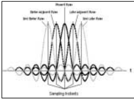
Figure 3. Interaction of raised cosine pulses when the time between pulses coincides with the data rate.
