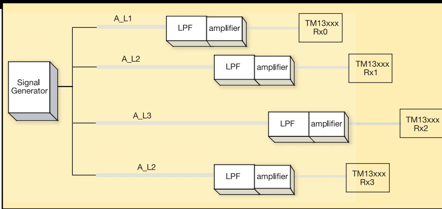
Figure 4. DFDS(S) system configuration.
