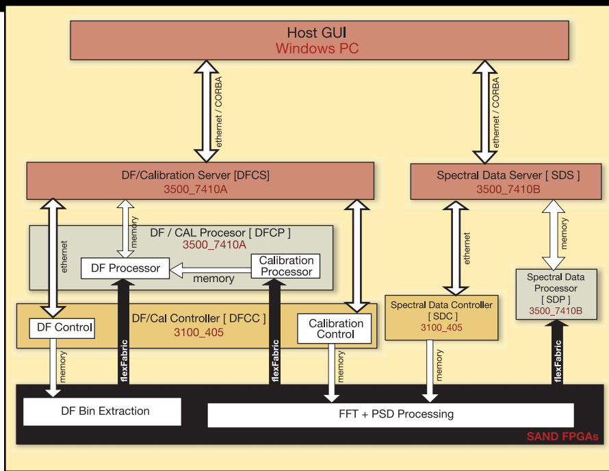
Figure 2. Software task mapping.
