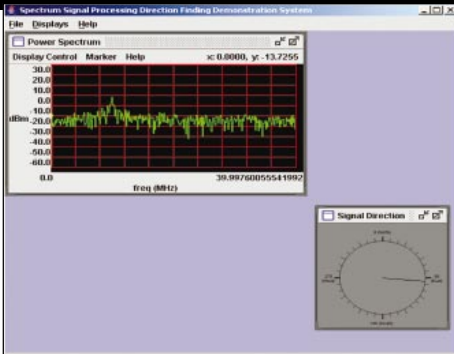
Figure 3. GUI display.
