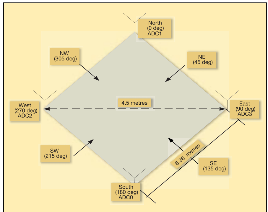
Figure 5. DFDS(T) system configuration.
