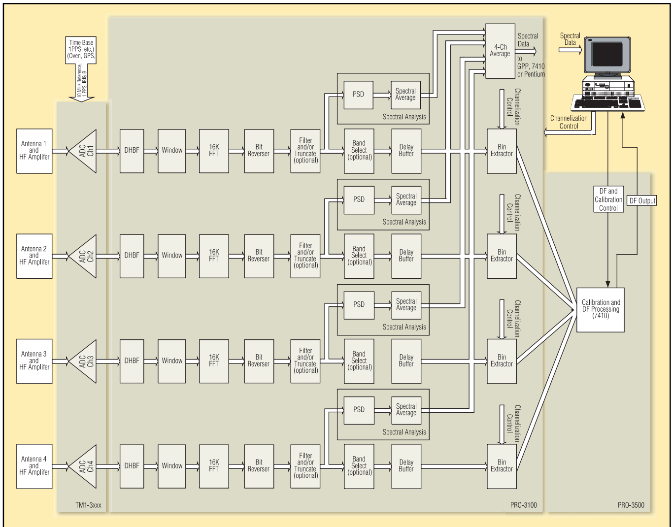
Figure1. Direction finding demonstration system processing blocks.
