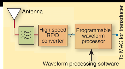
Figure 2. True software radio uses a single-carrier speed RF-to-digital converter to eliminate all analog front-end components. The output is then fed through proprietary filtering software and firmware.
