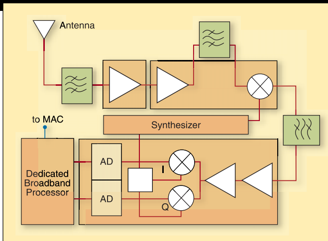
Figure 1. Up to now, SDR receivers depended on analog front ends to feed 70 MHz ADCs.
