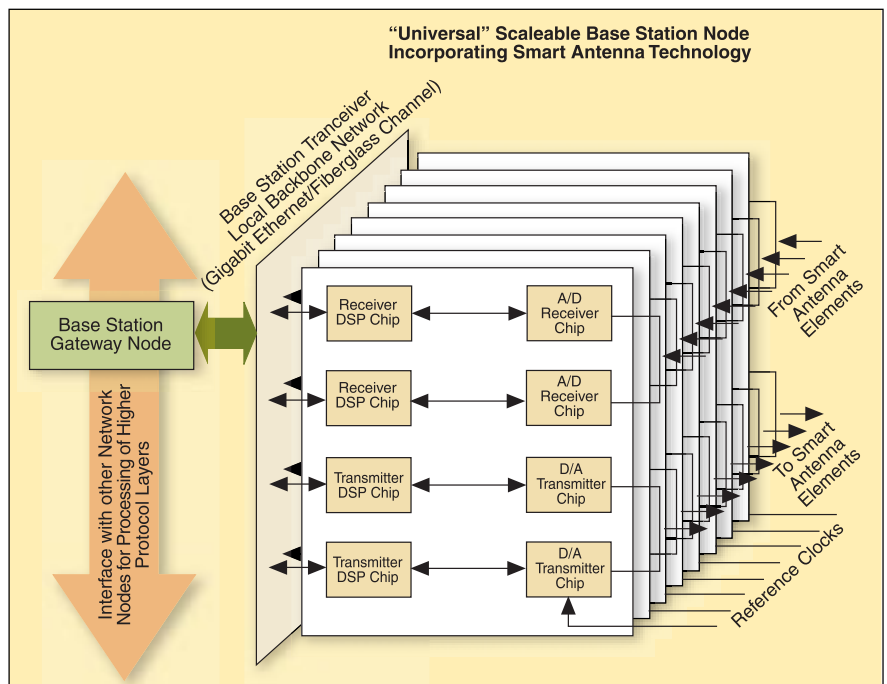
Figure 3. A scalable, electronically steerable antenna node (smart antenna).
